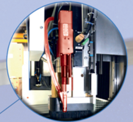
Screwing unit for automatic screw placement to fix the rotary shell to the support discs
