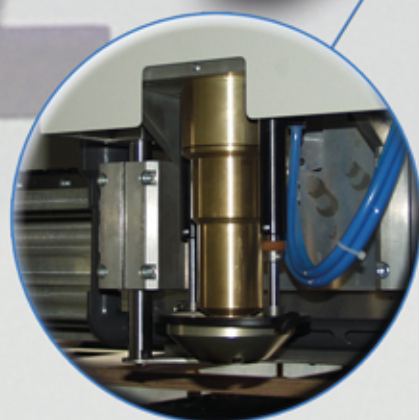
Standard cutting nozzle for the cutting of flat plywood
